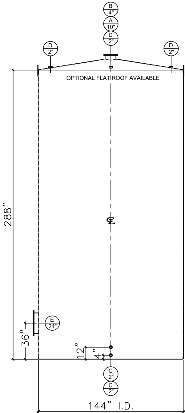
FRONT VIEW
