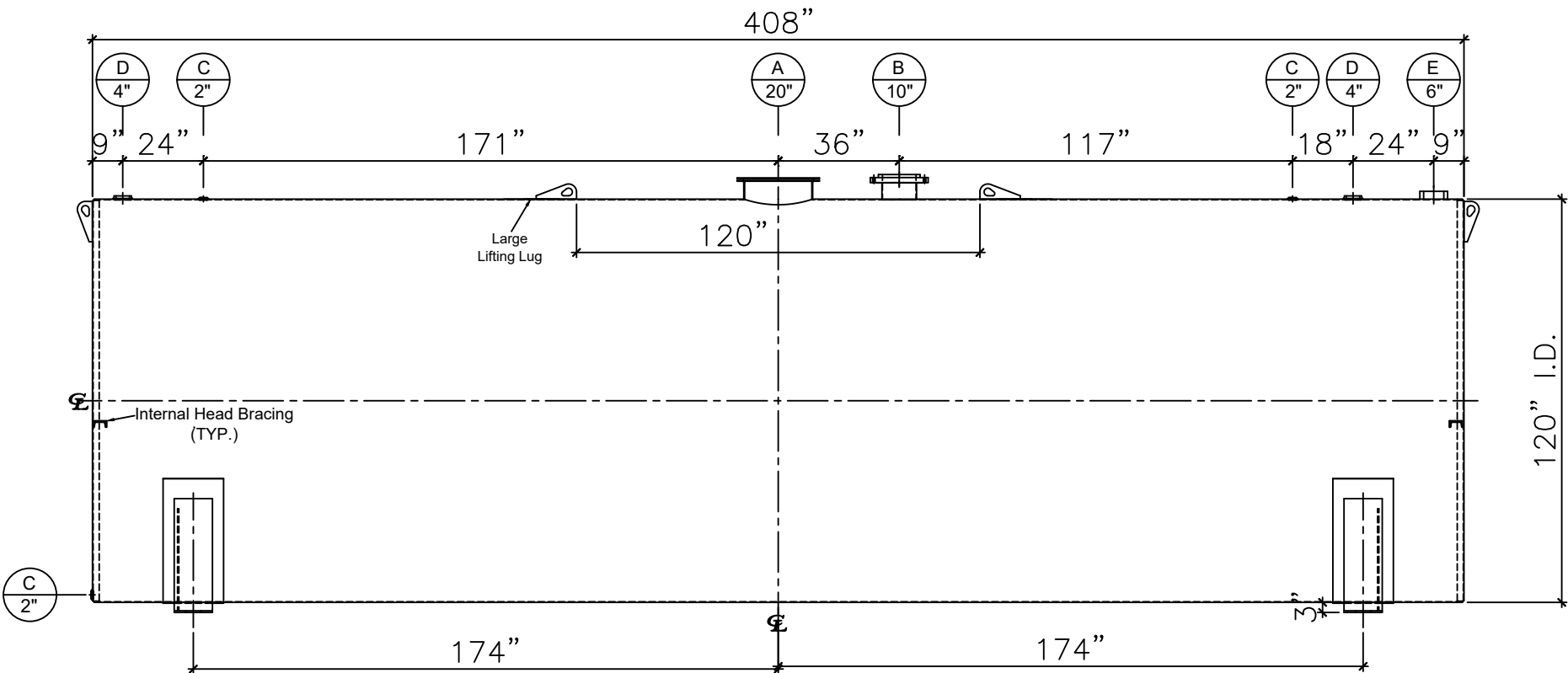
FRONT VIEW
