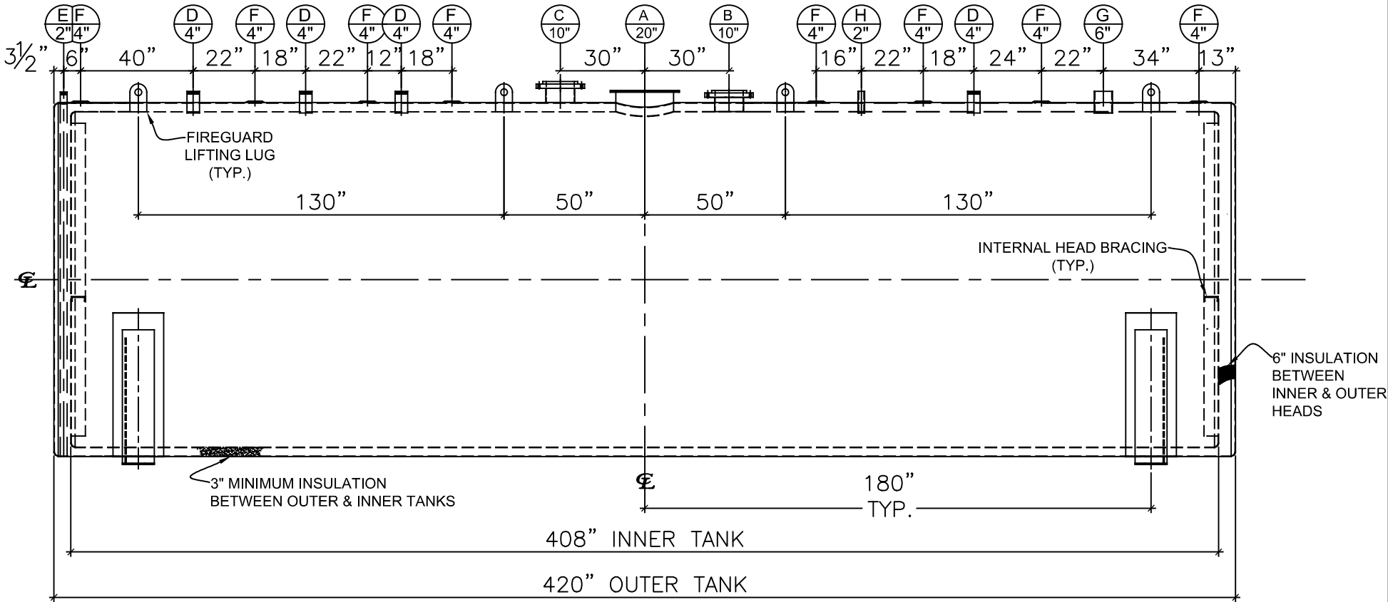
FRONT VIEW
