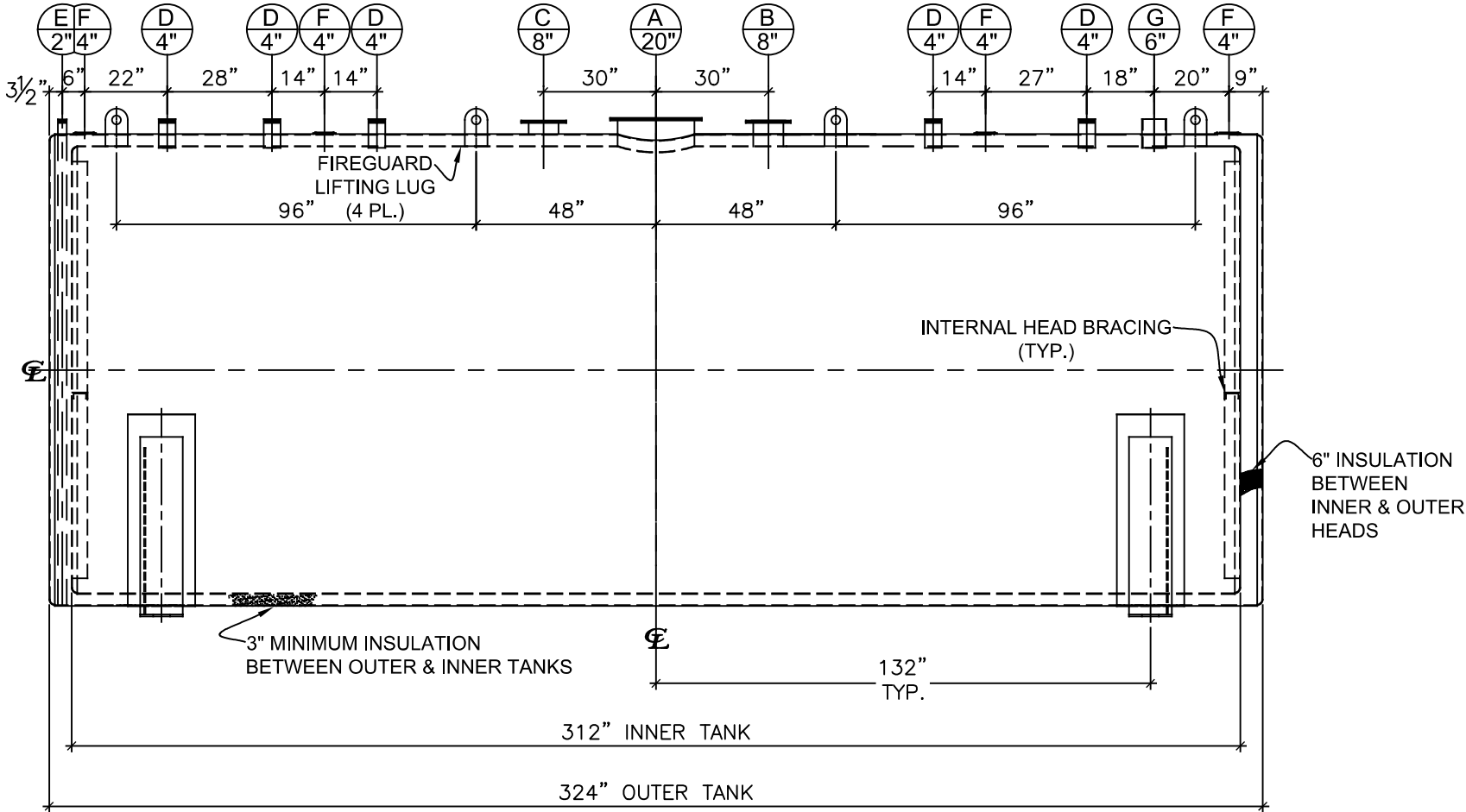
FRONT VIEW
