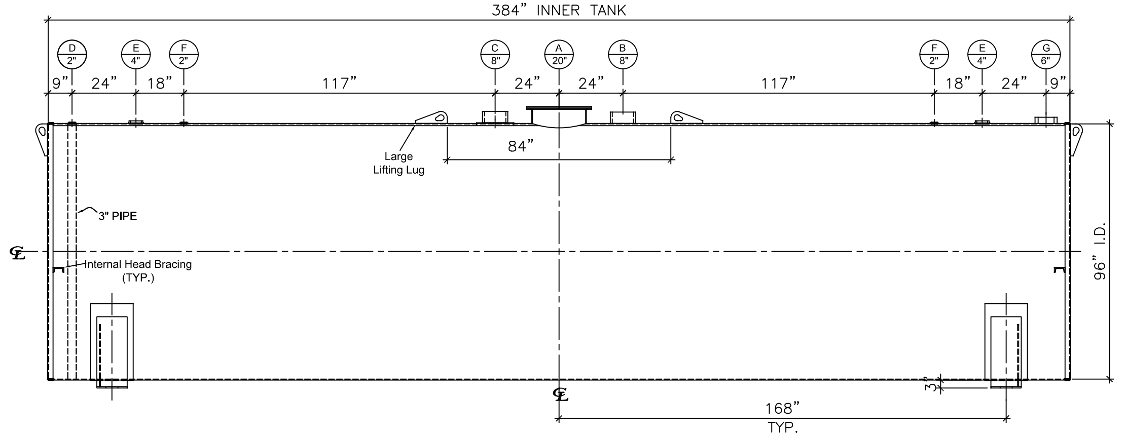
FRONT VIEW
