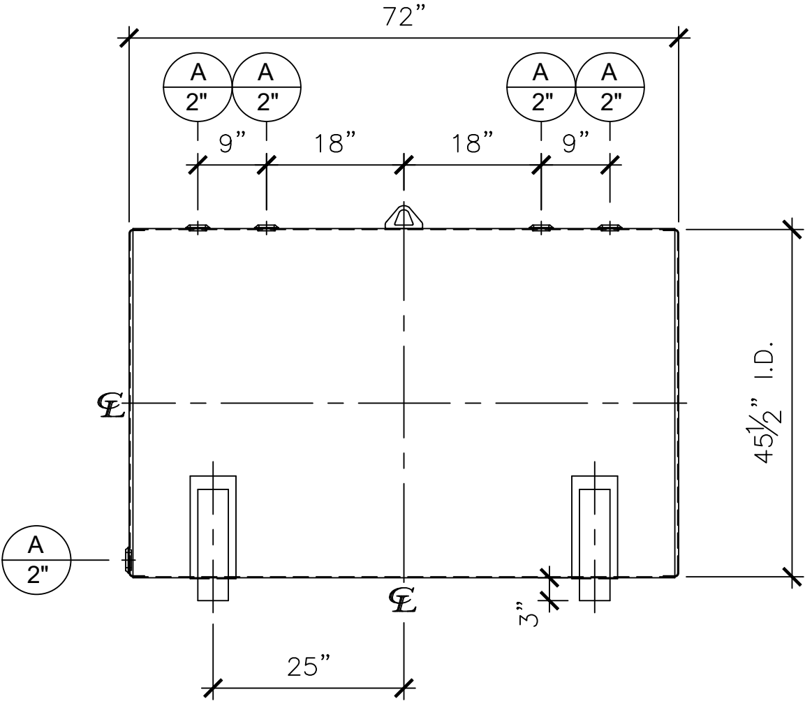
FRONT VIEW
