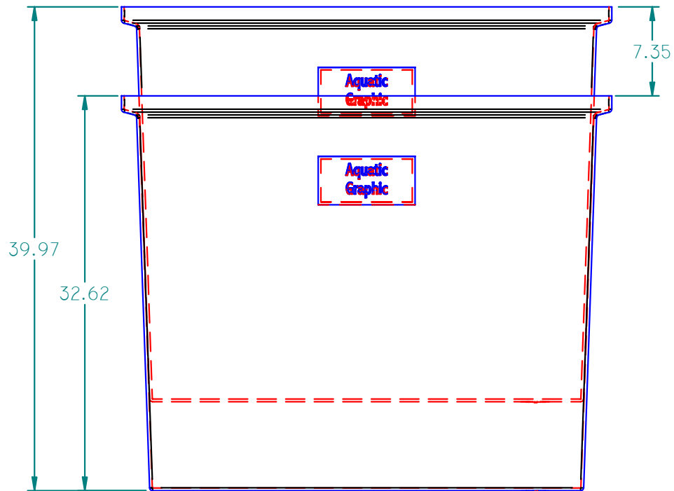
Side View Nested
