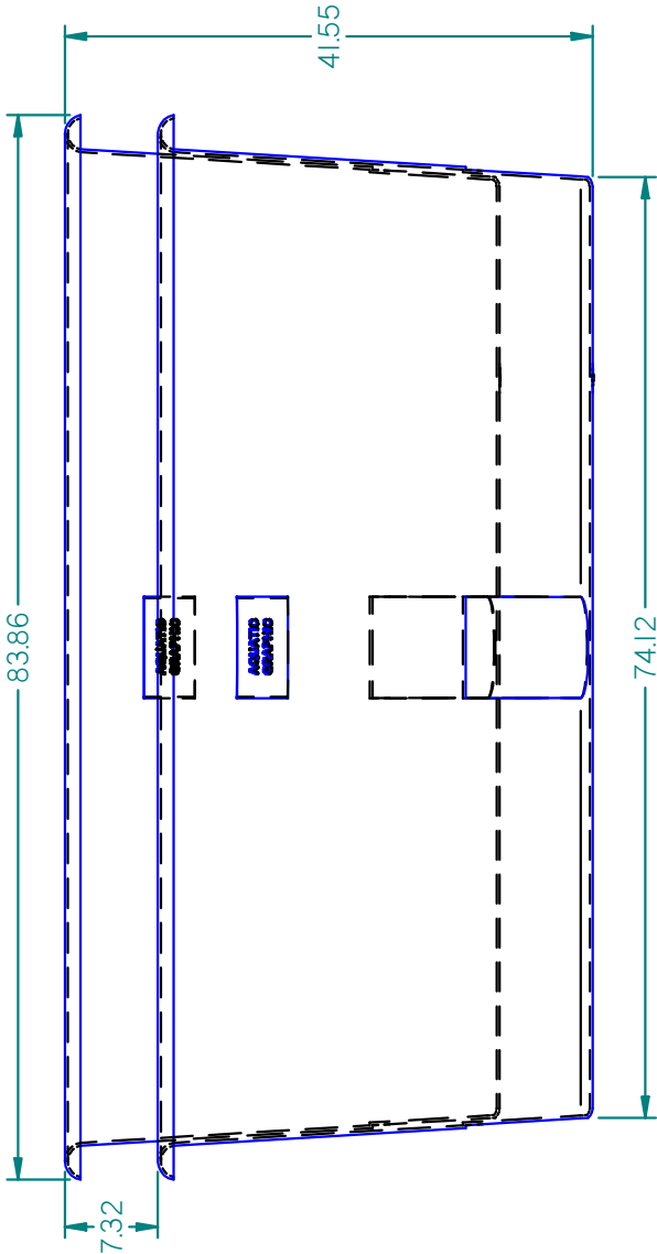
Nesting View
