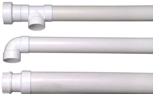
Two 3" diameter 6-ft. sections of pipe (for Downspout and Inlet connections) and one 4" diameter 6-ft. section of pipe (for Water Diverter Assembly)
